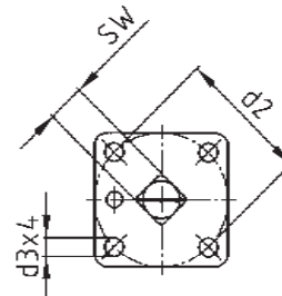
Montageflansch mounting flange
